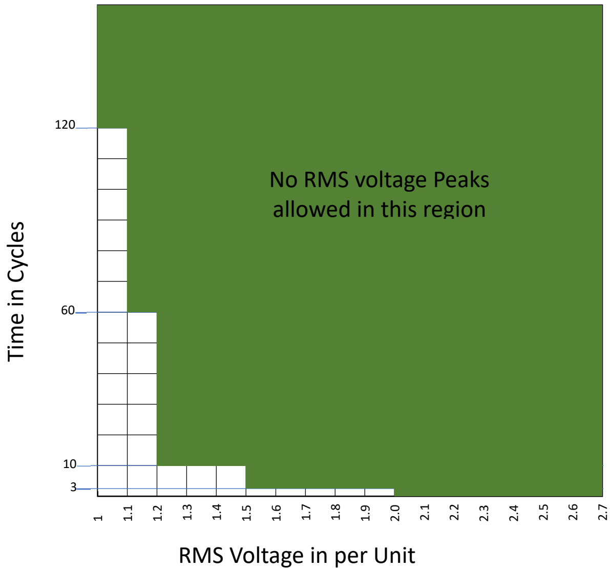
Figure 1 RMS Voltage Limits
